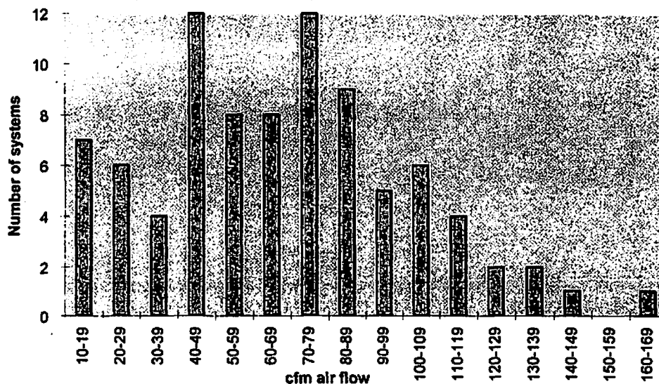
Figure 1 - ASD system Airflow from NJ study of mitigated houses
