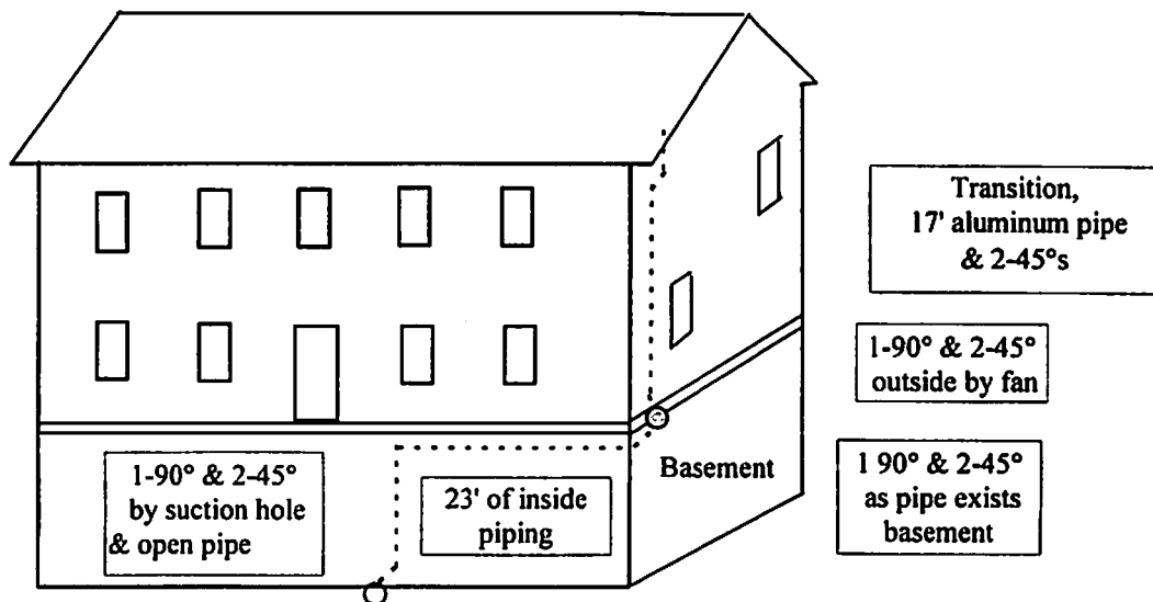
Figure 3 Example of a common ASD system with pipe routing up the exterior
