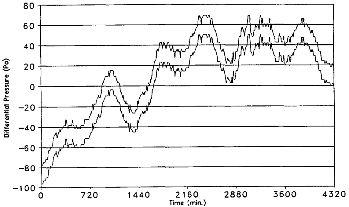
Figure 6: Prediction of wind-induced pressure differences in response to temporal variations in barometric pressure and indoor pressure equal to the average barometric pressure for 1 (upper curve) and 14 m/s wind on the leeward wall.
