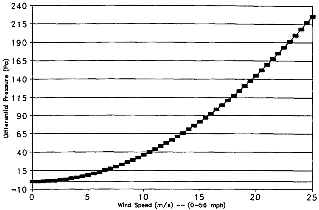
Figure 1: The wind-induced pressure differential predictions for a range of wind speed blowing on the windward side wall of a structure when the indoor pressure equals the barometric pressure.
