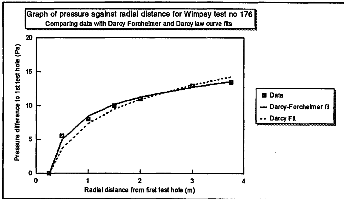
Figure 2: Typical pressure field result from Wimpey tests
