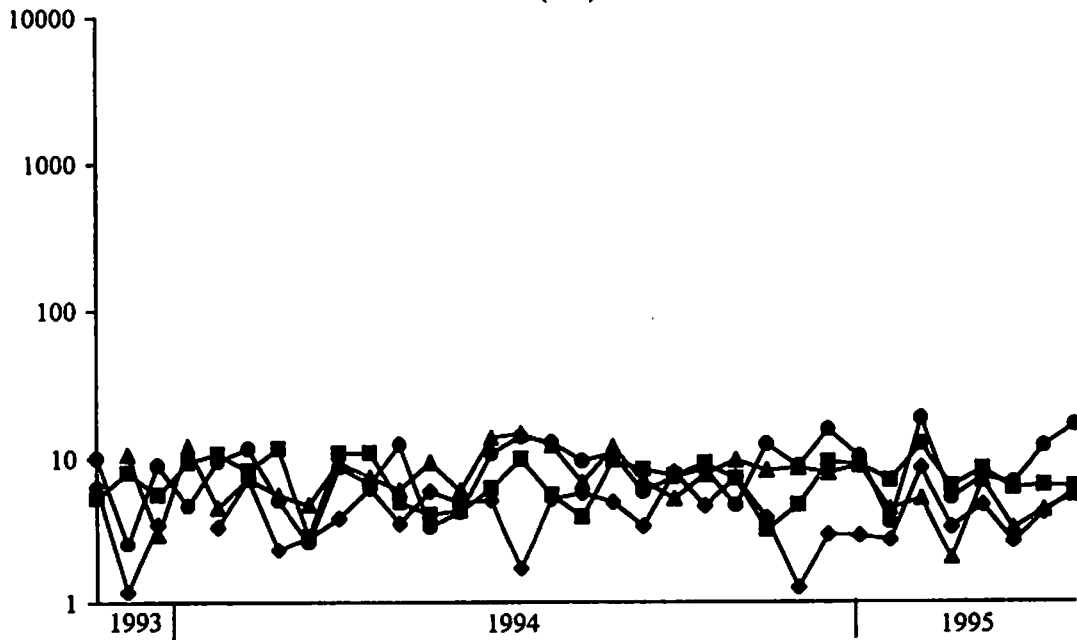
Fig. 6. ^{222}\text{Rn} (a) and ^{220}\text{Rn} (b) from the Aberdeen site position 4a obtained from 0.28, 0.56, 0.85 and 1.28 m depths from November, 1993 to March, 1995.
