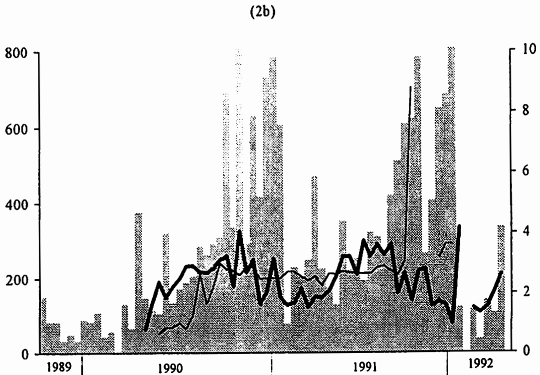
Fig. 2. ^{220}\text{Rn} , ^{222}\text{Rn} and permeability data from the Chester site obtained from 0.85 m depth tubes from September, 1989 to May, 1992. Position 1 data are shown in (a), (b) shows position 2 data, (c) shows position 3a data, (d) shows position 3b data, (e) shows position 4a data, (f) shows position 4b data, (g) shows position 5 data, and (h) shows position 6 data.
