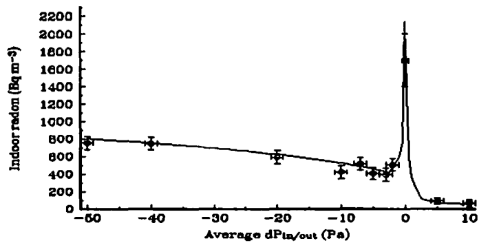
Figure 1: Time-averaged indoor radon concentrations as a function of whole house pressure conditions.
