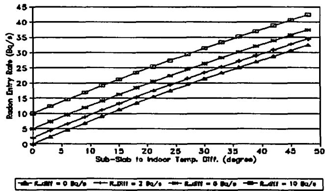
Figure 2: Predicted effects of temperature difference between the sub-slab and the indoors on the total radon entry rate when the indoor temperature is less than the sub-slab area temperature and equal to the outdoor temperature.
