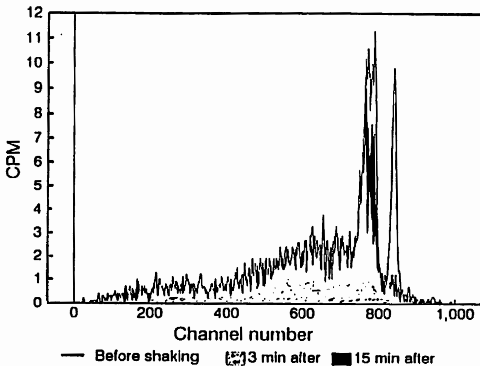
Fig. 1. Typical standard solution before and after shaking. The peaks above channel 800 ( ^{214}\text{Po } \alpha ) and the upper part of the composite peak below channel 800 ( ^{214}\text{Po } \alpha ) disappear upon shaking, then grow in gradually to restore the original spectrum.
