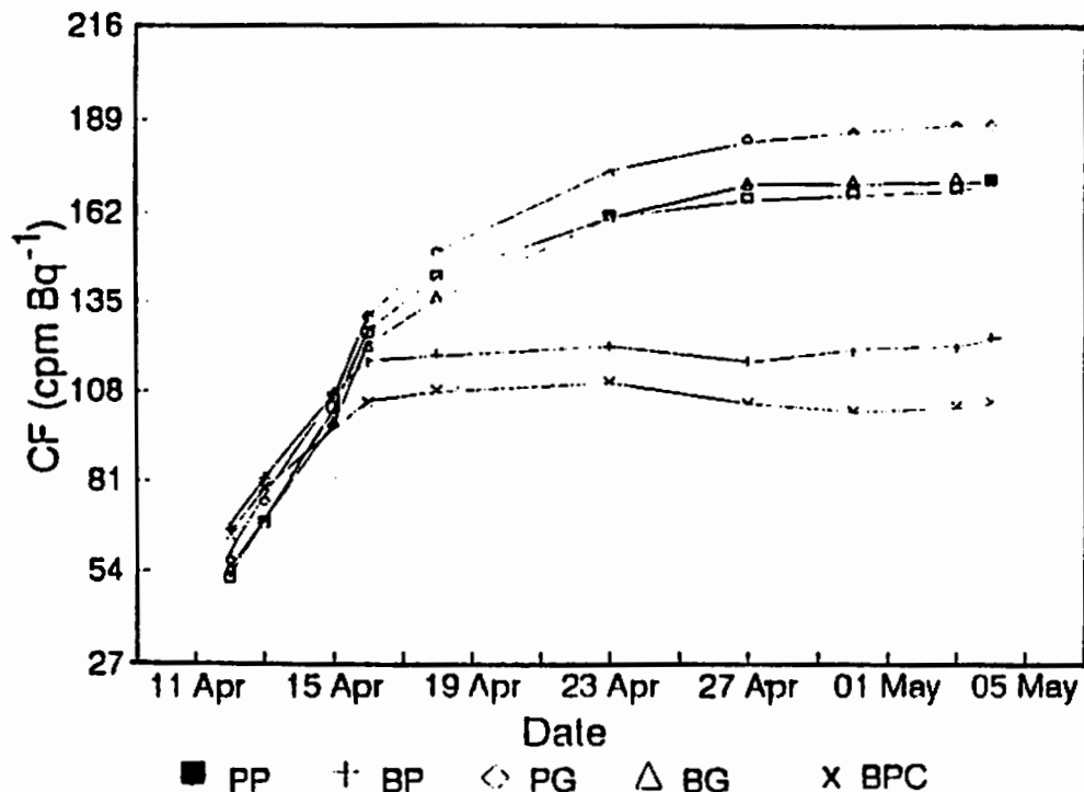
Fig. 8. Increase in conversion factors for two types of cocktail in two types of vial. Standards were prepared from Ra solution with (1) Packard Optifluor-C cocktail in plastic vials (PP), (2) Beckman Ready Organic cocktail in plastic vials (BP), (3) Packard cocktail in glass vials (PG), (4) Beckman cocktail in glass vials (BG), or (5) Beckman cocktail in plastic vials with added carrier (BPC).
