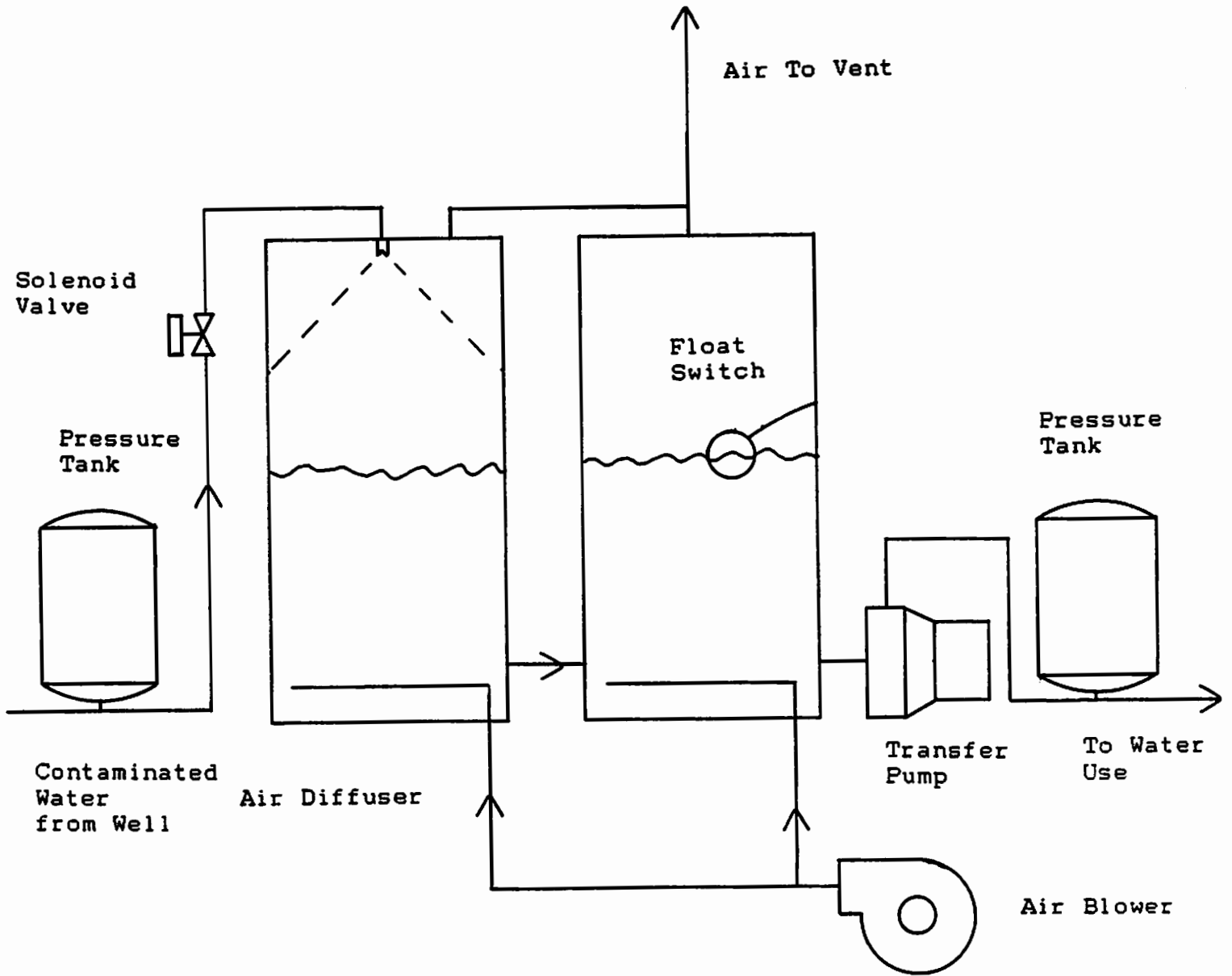
Figure 3. Diffused Aeration
