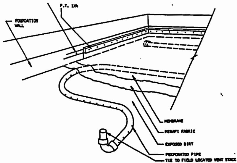
Figure 3. Crawlspace subliner ventilation
